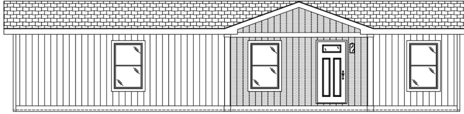
FRONT SIDEWALL W/ STANDARD NOMINAL 16'-0" DORMER
